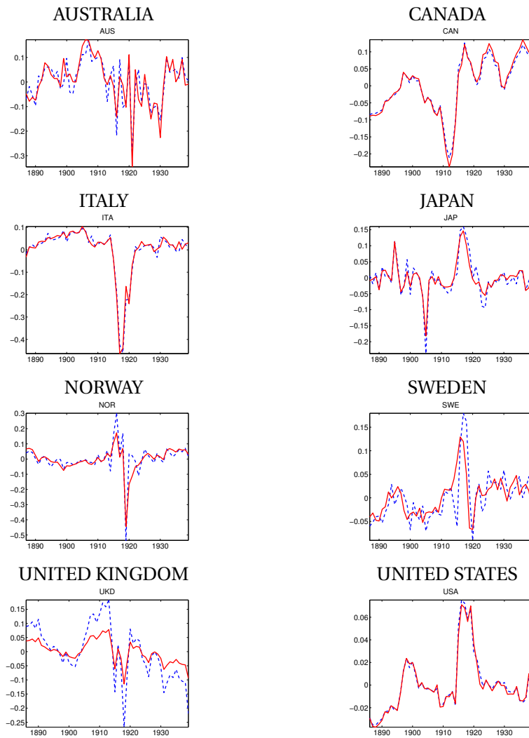
Figure 1: Actual current account/ net output ratio (solid, red line) vs. predicted current account (dashed line).
