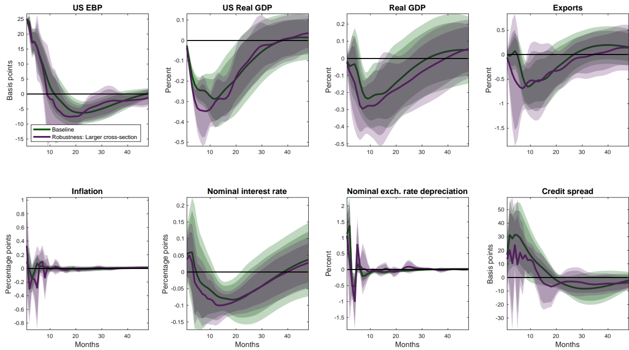
Figure A.3: Robustness: Larger Sample of Countries
